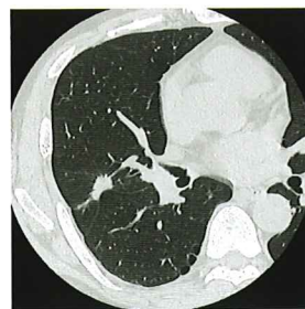
肺癌 (CT)
